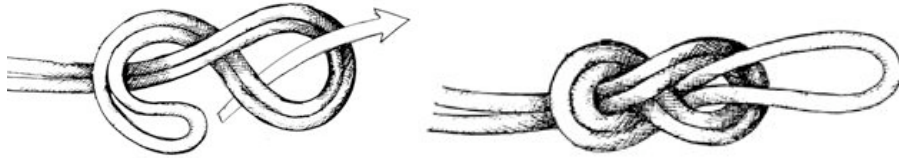
Tying a figure-of-eight on a bight
